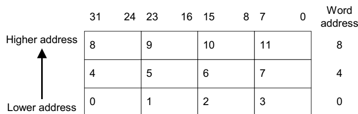
Figure 2-1 Big-endian addresses of bytes with words
